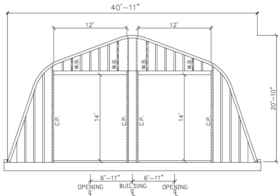
REAR ELEVATION
