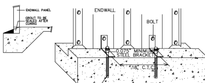
ENDWALL ANCHORAGE
