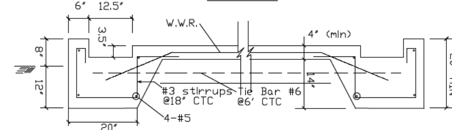
SEC B-B
