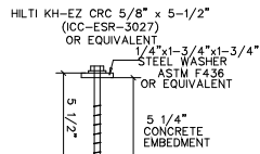
ANCHOR DETAIL
