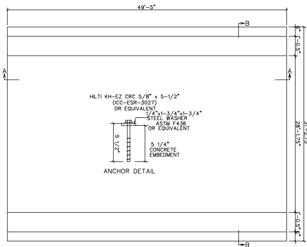
FOUNDATION PLAN
