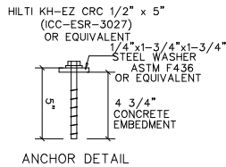
ANCHOR DETAIL
