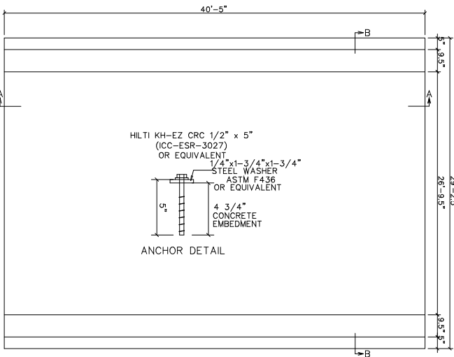
FOUNDATION PLAN
