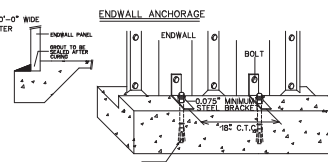
ENDWALL ANCHORAGE
