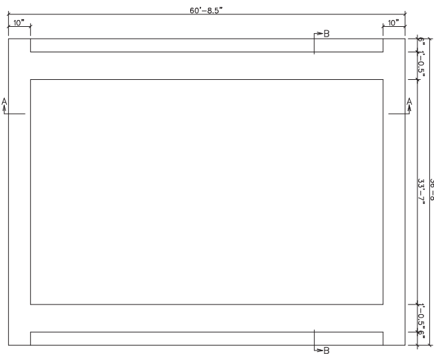
FOUNDATION PLAN
