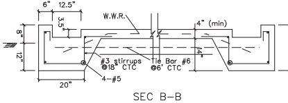
SEC B-B
