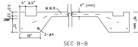
SEC B-B
