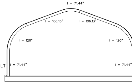
ARCH PROFILE
