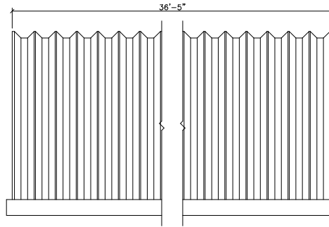
SIDE ELEVATION
