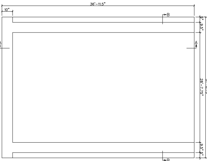
FOUNDATION PLAN
